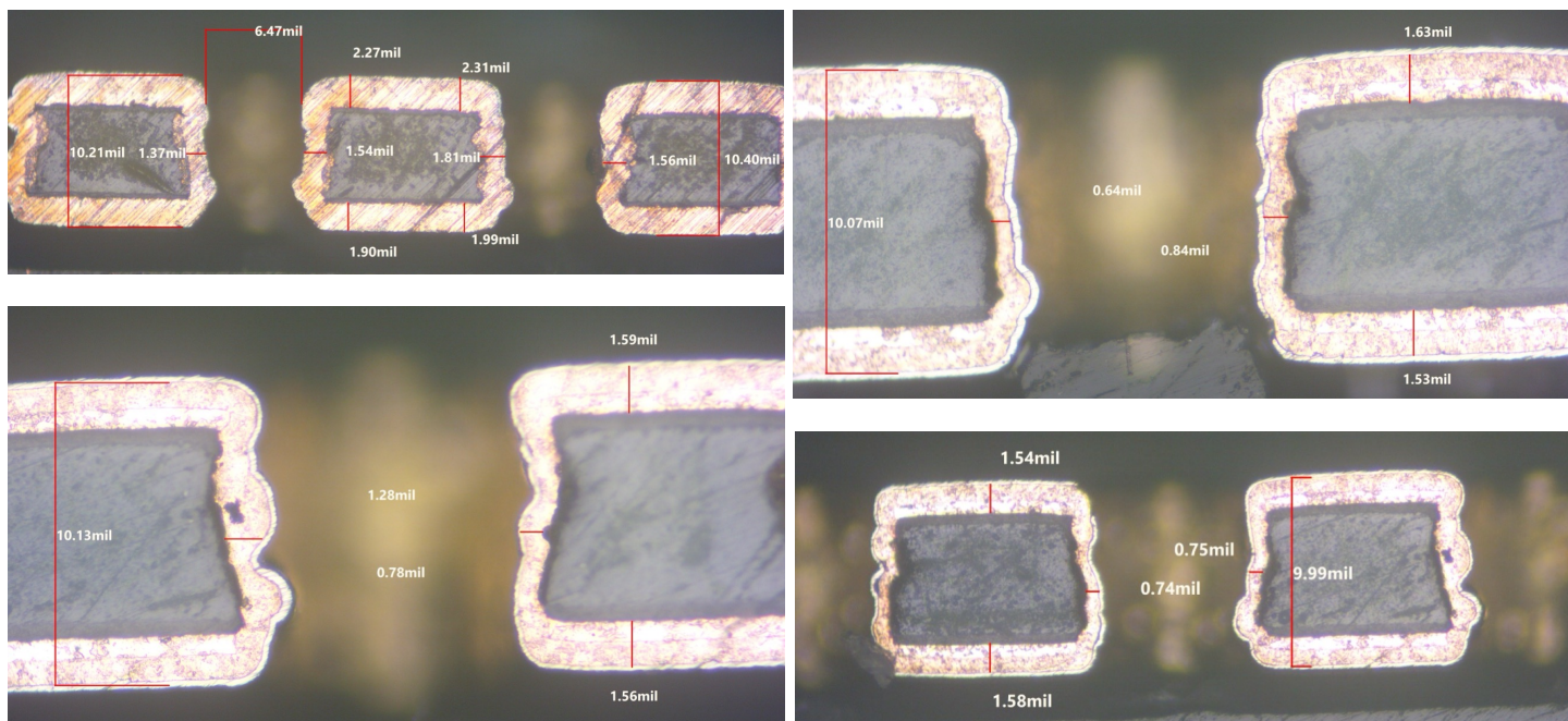
THESE VIAS SHOW TYPICAL DRILLING AND PLATING CHARACTERISTICS THAT VALIDATE PHASEBLUE'S ABILITY TO PRODUCE RELIABLE THRU HOLES
